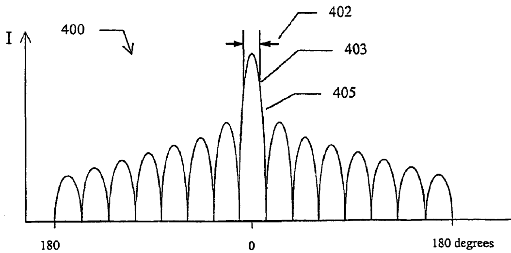
Figure 2B: Azimuth Beamwidth
