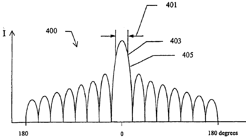
Figure 2A: Elevation Beamwidth
