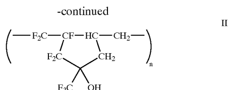
[0108] FIG. 6 Fluoroalcohol Polymers Made from Polymerization of Either Alicyclic Moieties (I) or Fluorinated Dienes (II)
