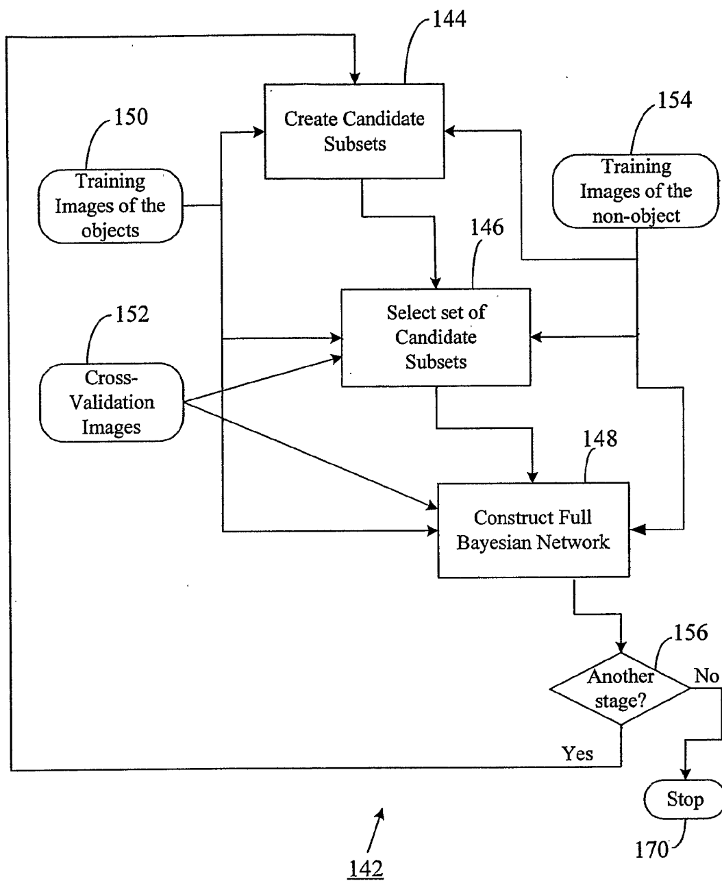
System for Creation of Bayesian Network Classifier
