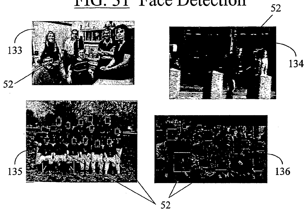
FIG. 31 Face Detection
