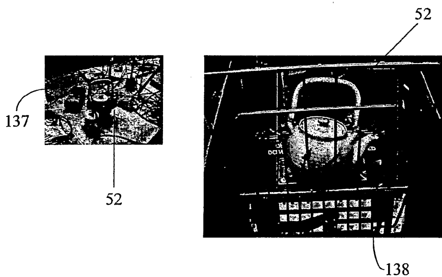
FIG. 32 Teapot Detection
