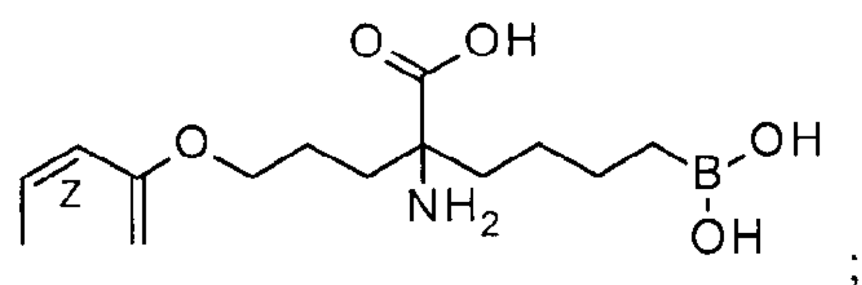
2-Amino-6-borono-2-(4-phenylbutyl)hexanoic acid:
