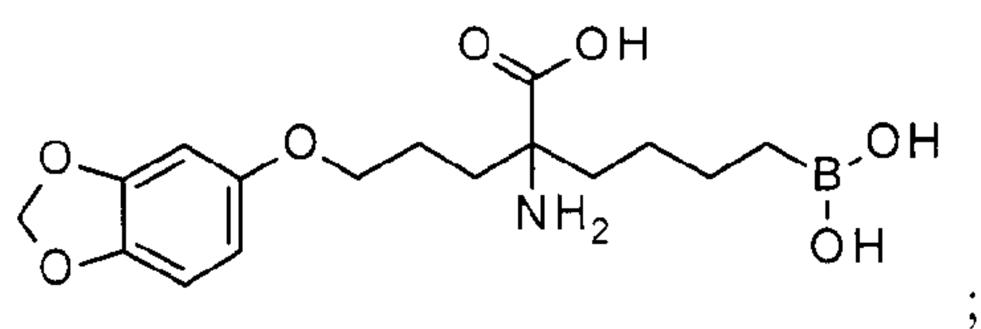
2-Amino-2-(3-(benzo[d][1,3]dioxol-5-yloxy)propyl)-6-borohexanoic acid:
