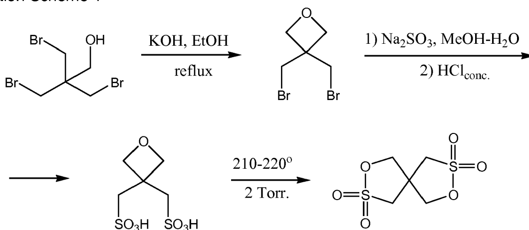
Reaction Scheme 1
