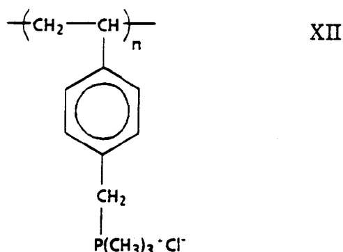
poly(vinyl benzyl trimethyl phosphonium chloride)
