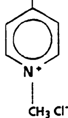
poly ( N- methylvinylpyridinium chloride )
