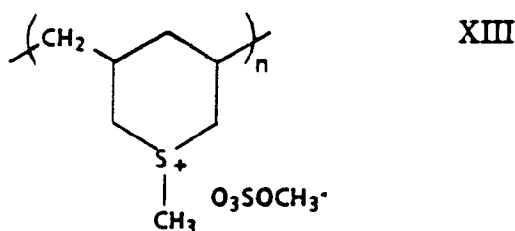
poly(methyldiallyl sulfonium methylsulfate)
