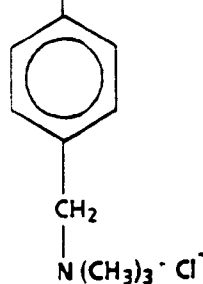
poly (vinyl benzyl trimethyl ammonium chloride )
