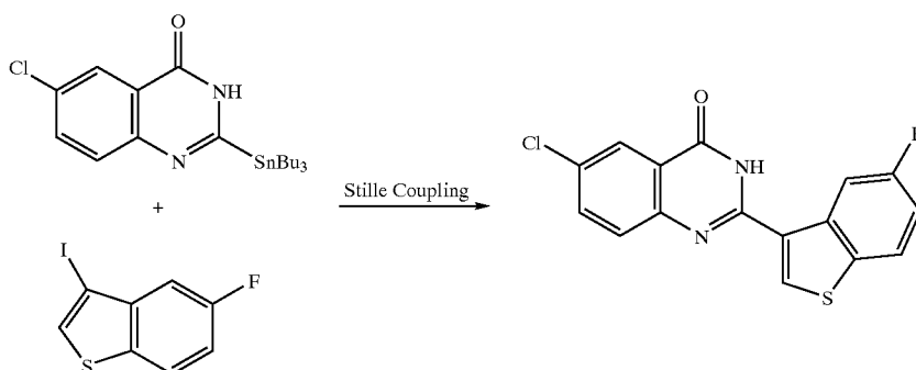
Stille Coupling No. 2
