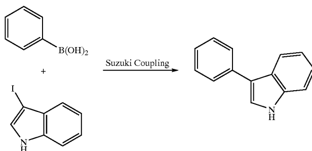
Suzuki Coupling No. 2:
