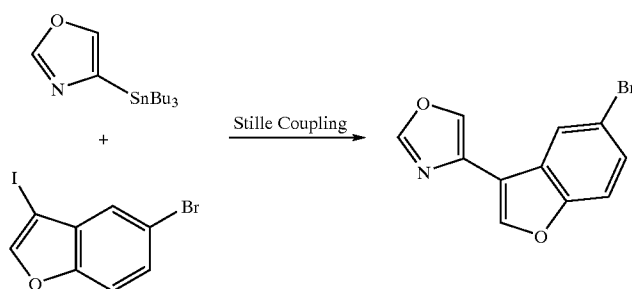
Stille Coupling No. 2
