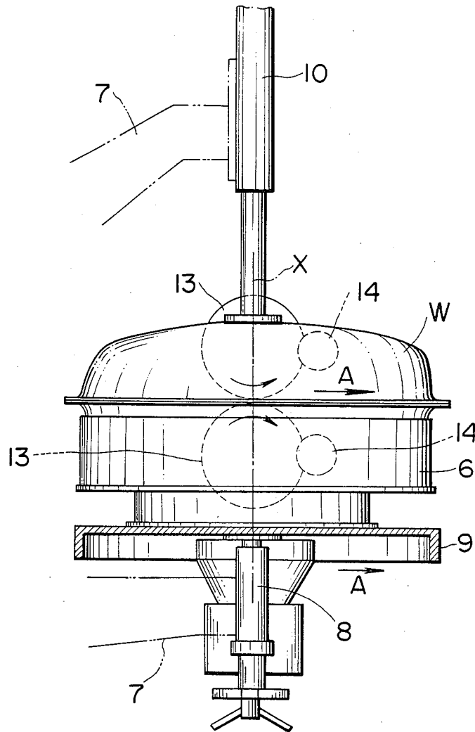
FIG. 4 (PRIOR ART)
