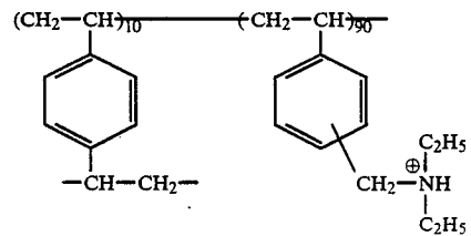
Dye Compound D (Comparison Dye D)
