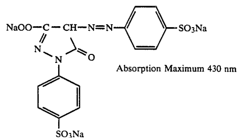
Nucleating Agent (Comparison compound (c))
