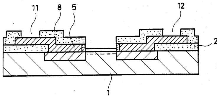
FIG.4G PRIOR ART
