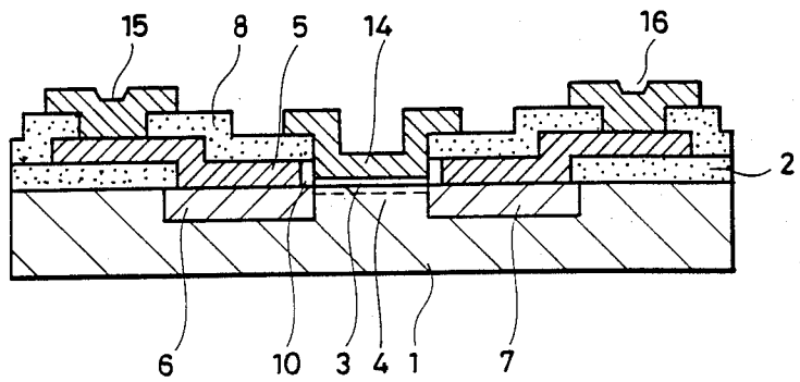
FIG.4G PRIOR ART
