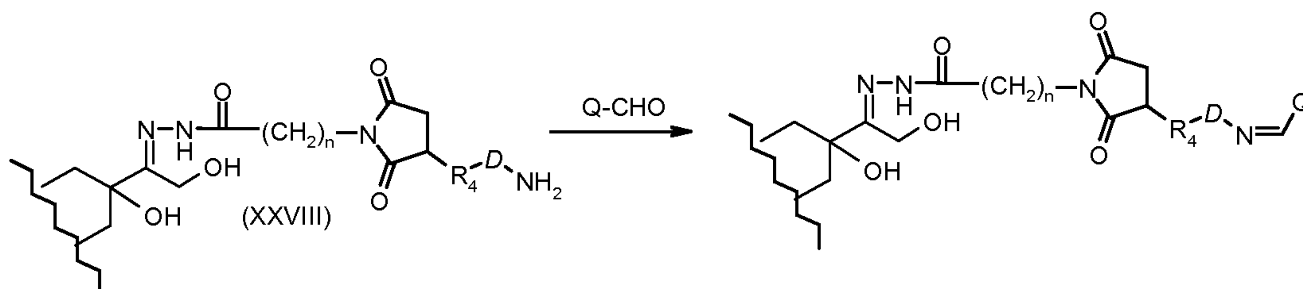
Scheme 13
