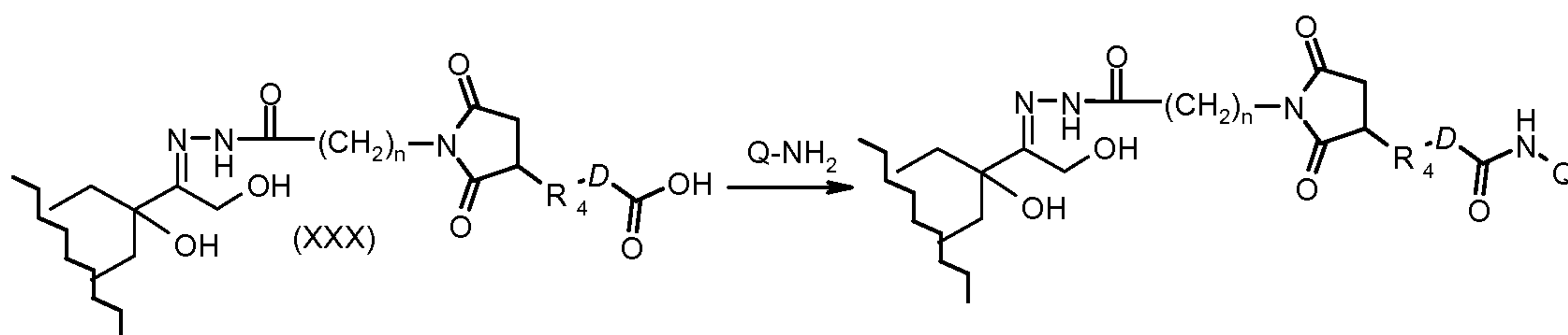
Scheme 12
