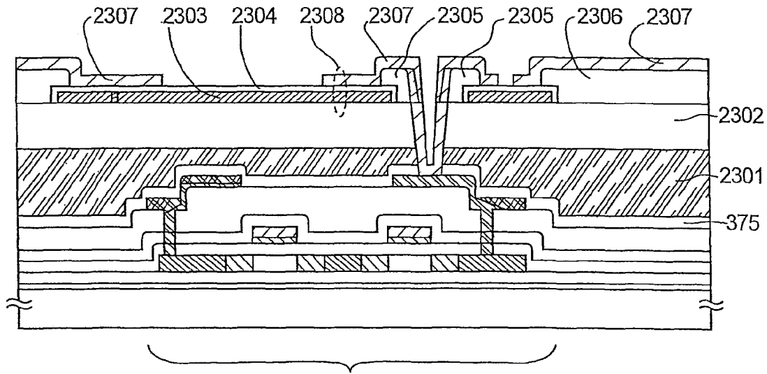
701: n-CHANNEL TFT
