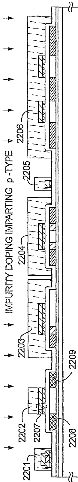
FIG. 22B FORMING p++ REGION
