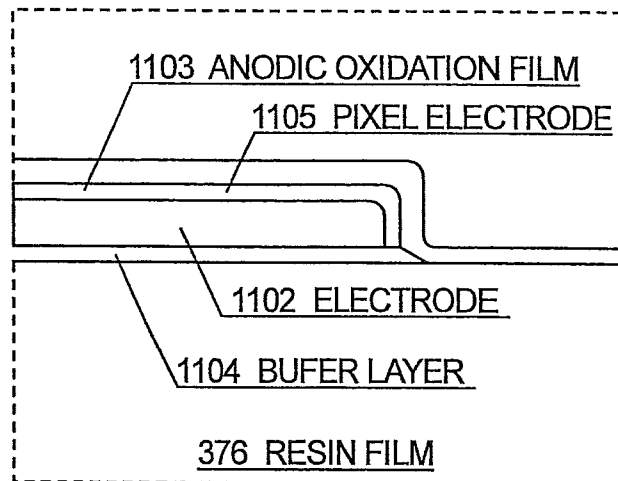
SCHEMETIC DIAGRAM OF ENLARGED ELECTRODE EDGE PORTION
