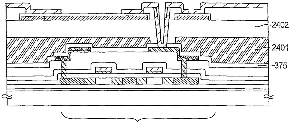
701: n-CHANNEL TFT
