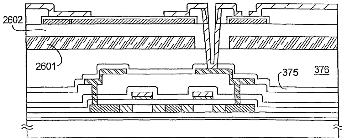
701: n-CHANNEL TFT
