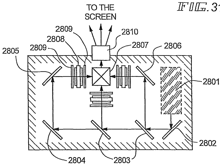
PROJECTION DEVICE (THREE PLATE TYPE)
