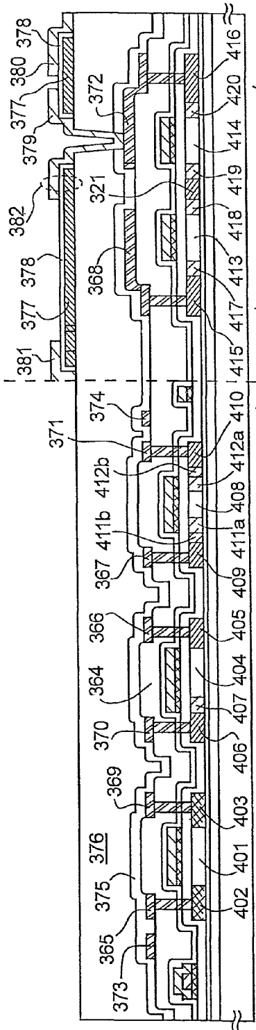
501: p-CHANNEL TFT 502: n-CHANNEL TFT 503: n-CHANNEL TFT 504: n-CHANNEL TFT DRIVER CIRCUIT PIXEL MATRIX CIRCUIT FIG. 5C
