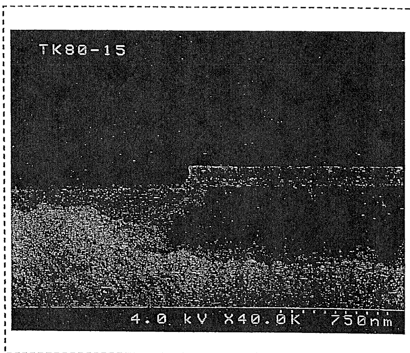
FIG. 1A SEM PHOTOGRAPH (CROSS SECTION)
