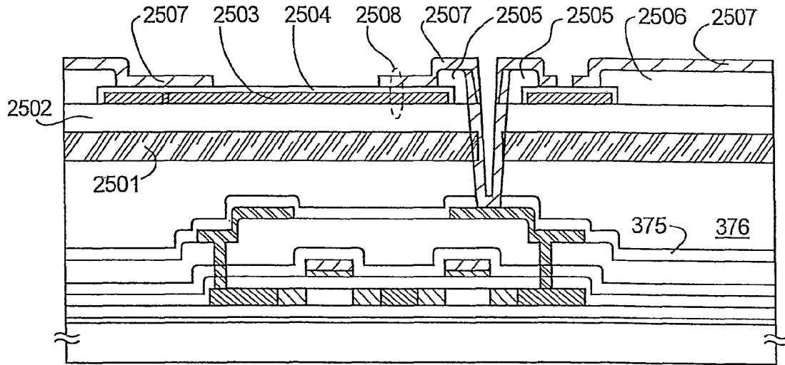
701: n-CHANNEL TFT
