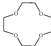
12-crown-4 ether (C-2)
