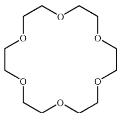
18-crown-6 ether
