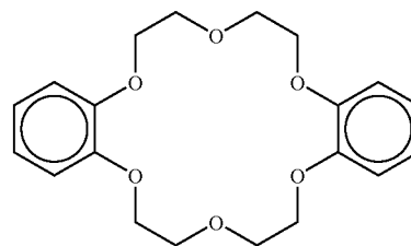
dibenzo-18-crown-6 ether (C-4)
