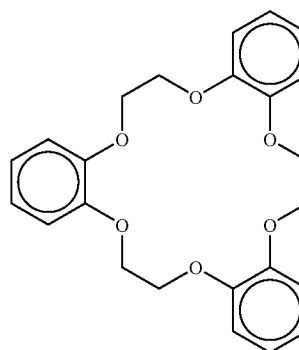
tribenzo-18-crown-6 ether (C-5)
