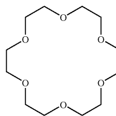
18-crown-6 ether (C-3)
