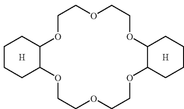
perhydrobenzo-18-crown-6 ether (C-7)
