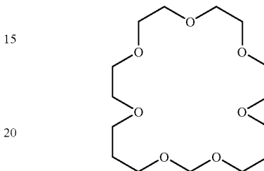
21-crown-7 ether
