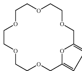
18-crown-6 furan (C-6)
