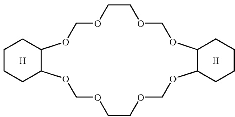
18-crown-6 ether
