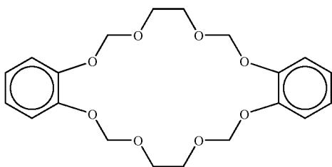
dicyclohexano-24-crown-8 ether (C-10)
