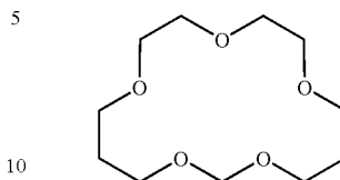
21-crown-7 ether
