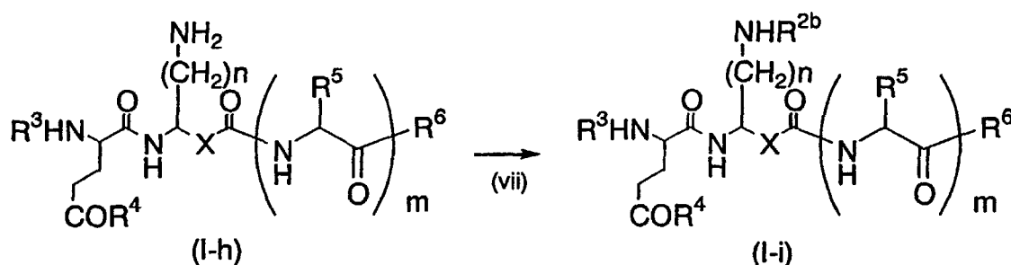
[Reaction Scheme 6]
