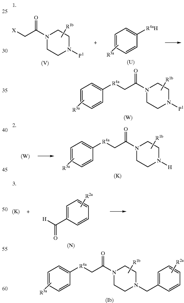
Reaction Scheme 6
