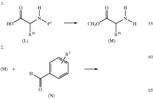
Reaction Scheme 4
