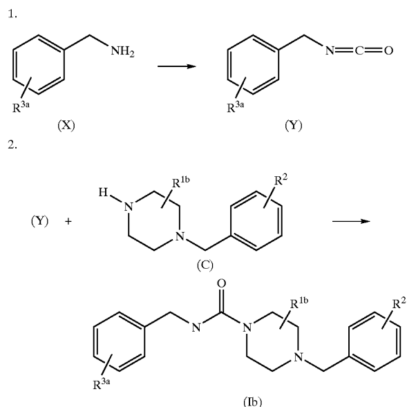
Reaction Scheme 7
