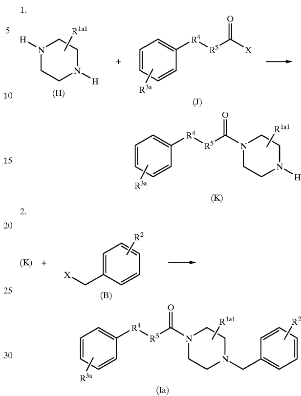
Reaction Scheme 3
