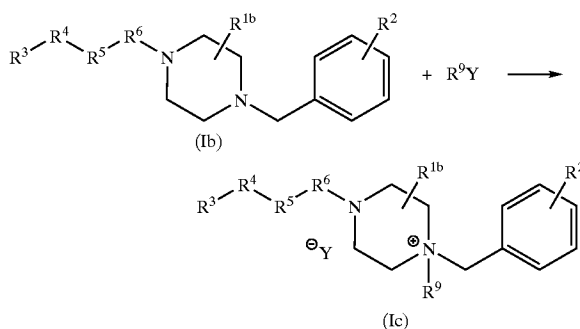
Reaction Scheme 8
