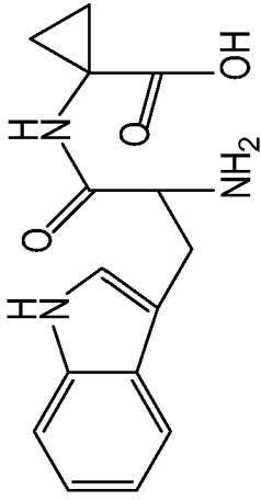
H 2 N-Trp-cyclopropane-OH
