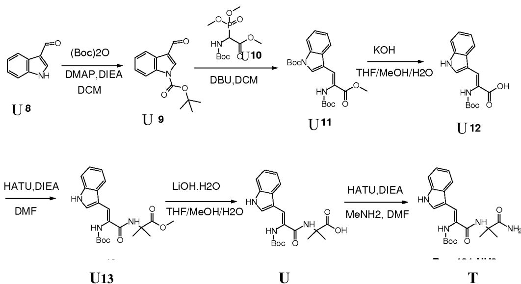
Scheme 4
