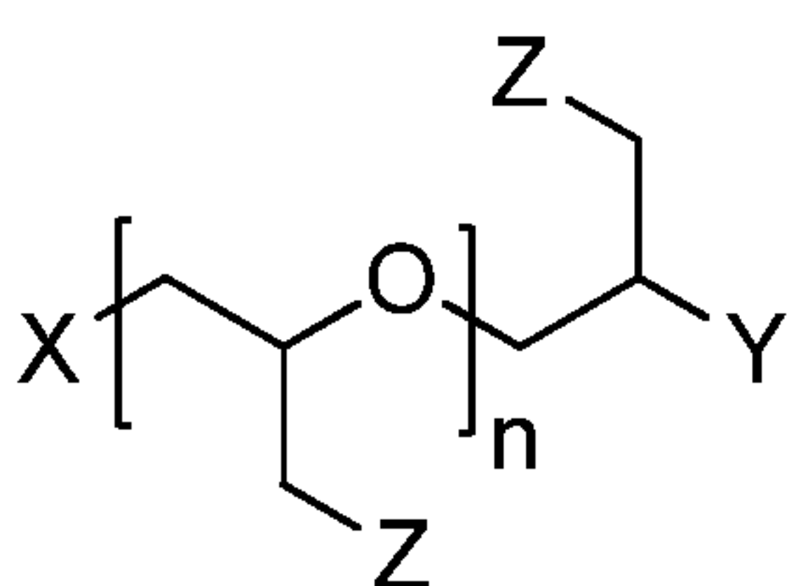
1,2-linked linear polyglycerol
