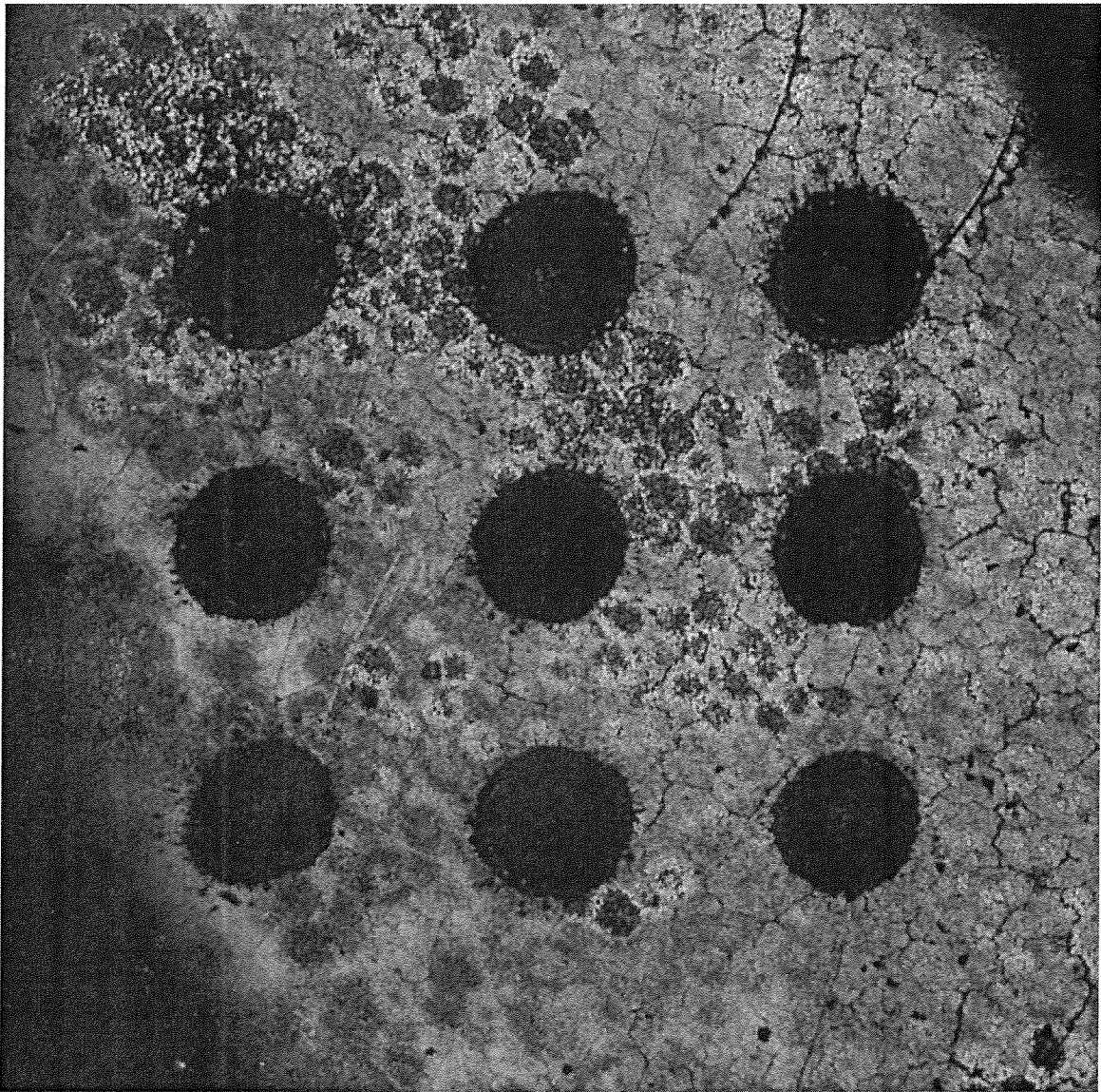
40uS ON-Time, 10 Pulses per Crater
