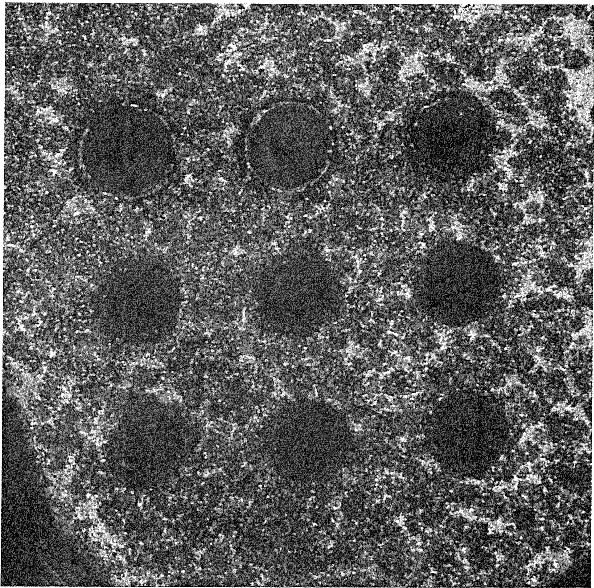
40uS ON-Time, 30 Pulses per Crater
