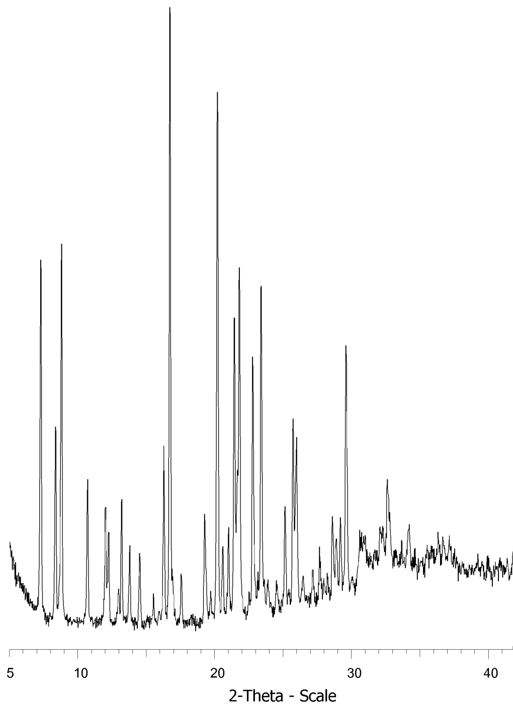
Figure 1. [Compound 1.HCl.3H 2 O] adduct XRPD spectrum.
