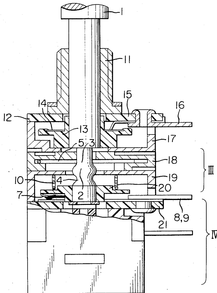
FIG. 3 PRIOR ART
