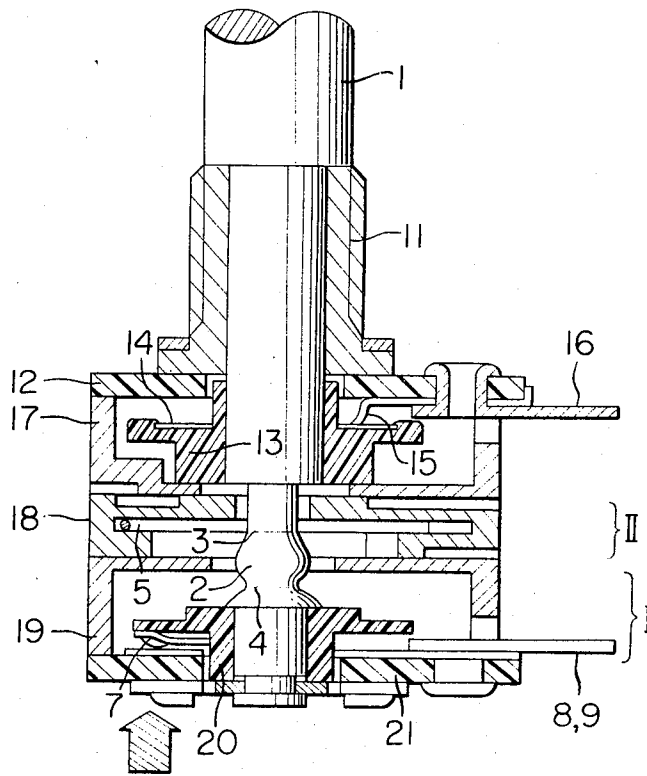
FIG. 2 PRIOR ART
