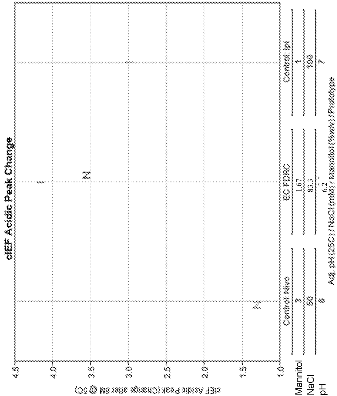
Fig. 2B: 1:1 Ratio Fixed Dosing Formulation for Nivolumab and Ipilimumab Charge Profile Change (cIEF) (6M at 5°C)
