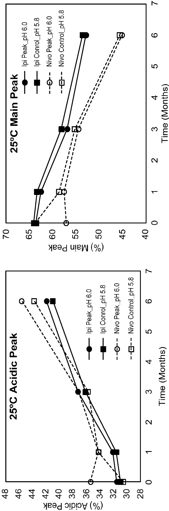
Figure 19. cIEF Peak Profile: Impact of pH
