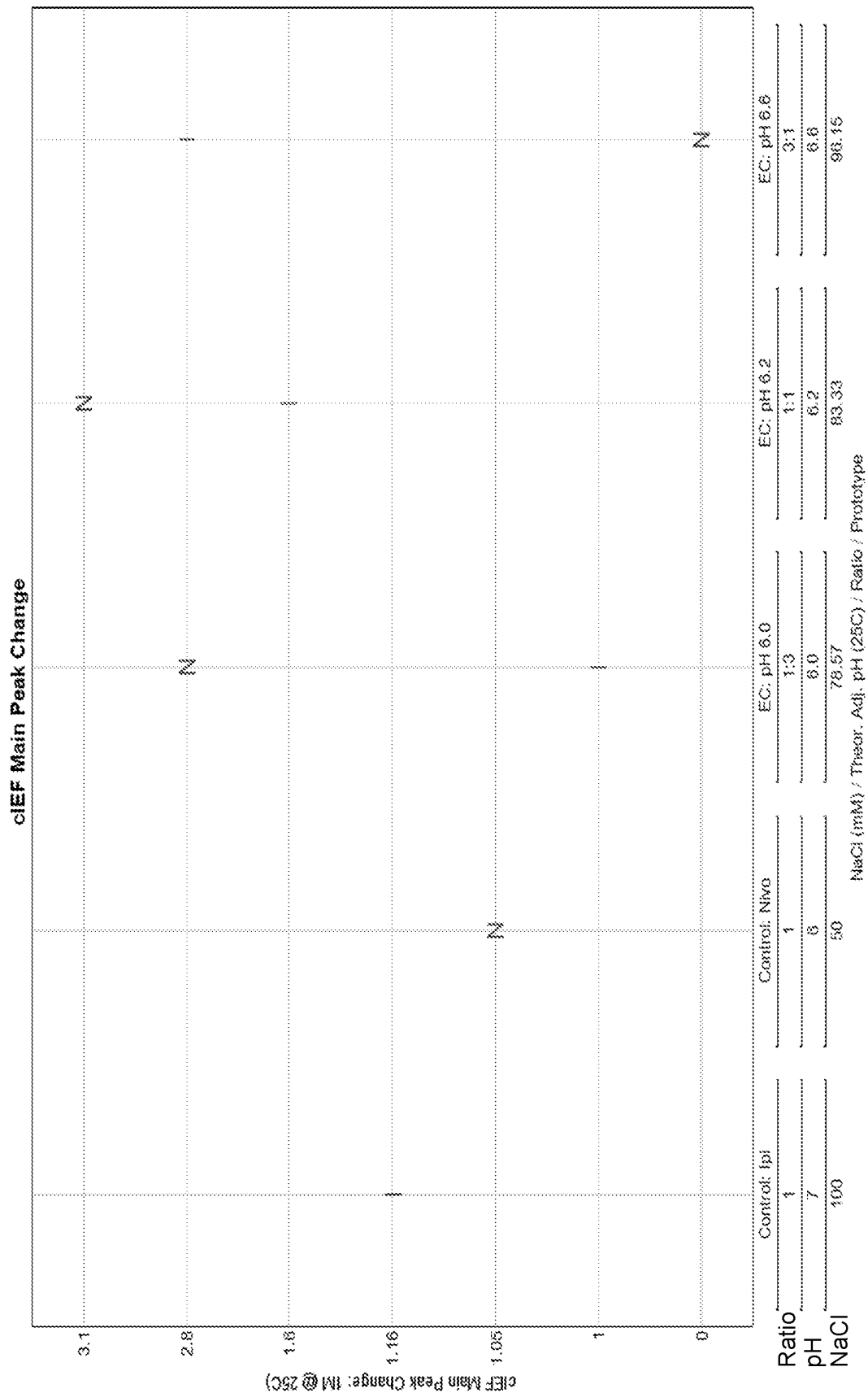
Fig. 4C: 1:3, 1:1, 3:1 Fixed Dosing Formulations for Nivolumab and Ipilimumab: cIEF Acidic Peak Change (1M at 25°C)
