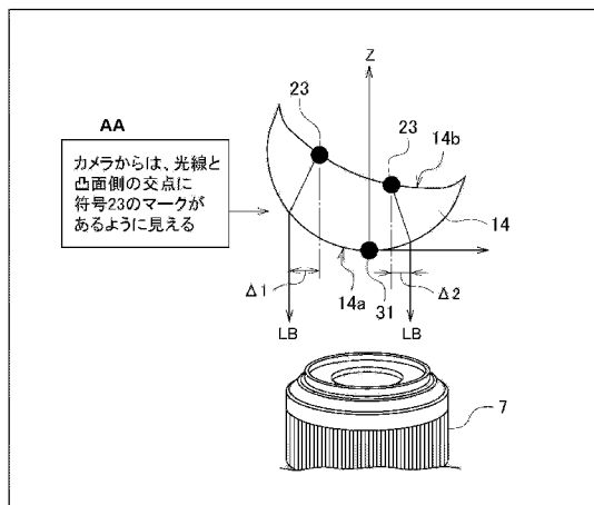
AA From the camera, the marks at symbols (23) appear to be located at the intersection between the light beam and the convex surface
