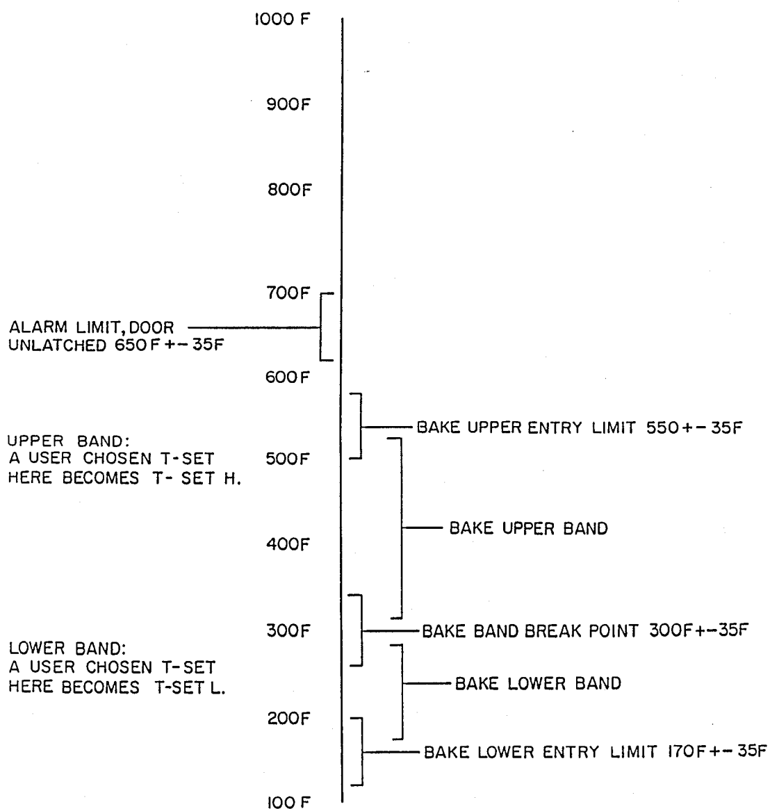
BAKE MODE TEMPERATURE ACTION POINTS.
