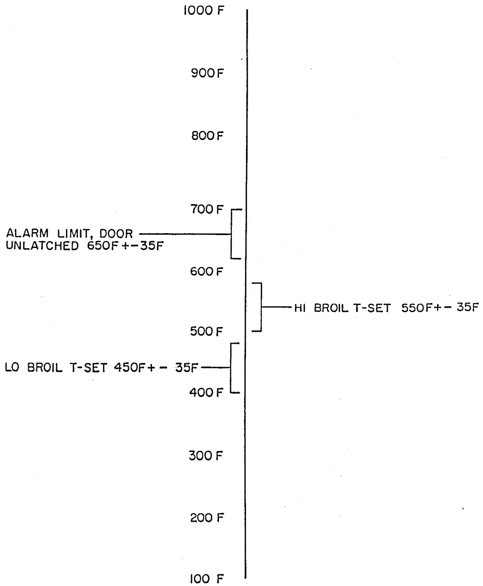
BROIL MODE TEMPERATURE ACTION POINTS.
