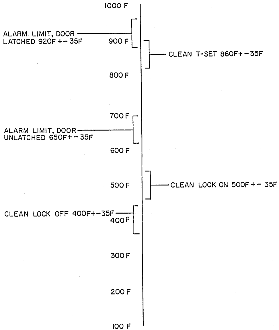
CLEAN MODE TEMPERATURE ACTION POINTS.
