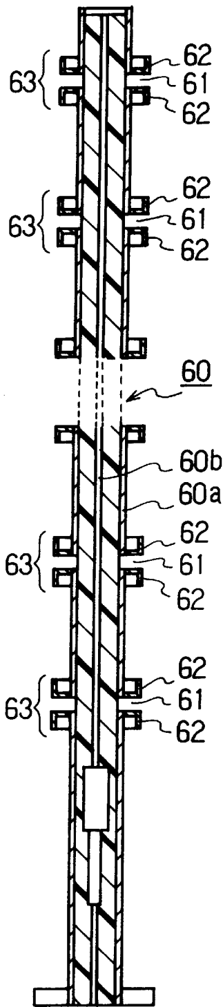
FIG. 17 (PRIOR ART)
