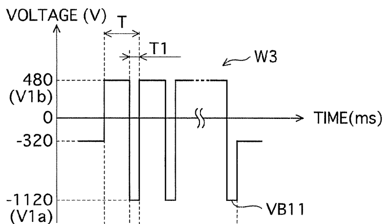
FIG.5B SUPPLY BIAS
