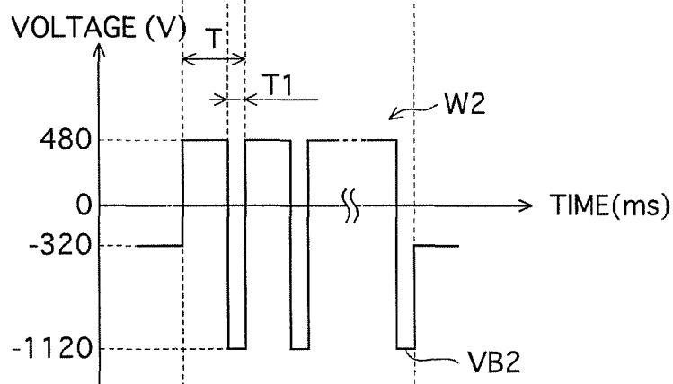
FIG.4B SUPPLY BIAS
