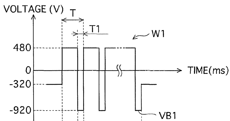
FIG.4A DEVELOPING BIAS
