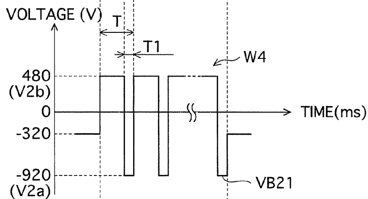
FIG.5B SUPPLY BIAS
