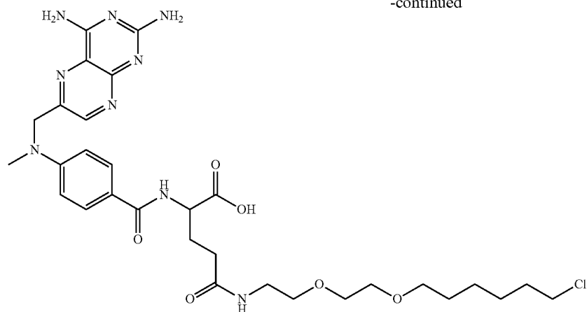
PBI-4848: Methotrexate-O2 chloroalkane
