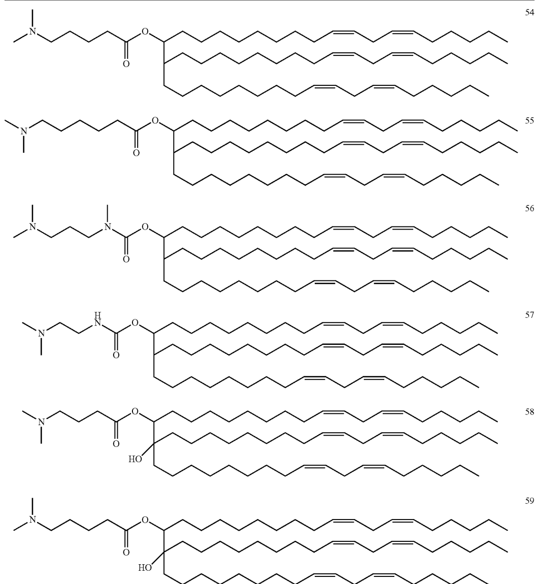
structures of long chain trialkyl cationic lipids
