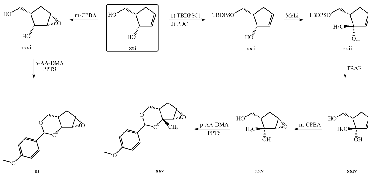
Scheme 3: Synthesis of substituted epoxides
