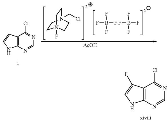
Scheme 8: Synthesis of 5-fluoro pyrrolo[2,3-d]pyrimidines
