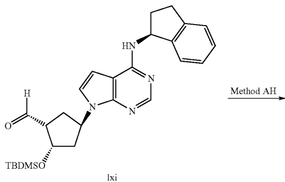
Scheme 12: Synthesis of (E)-2-((1S,2S,4R)-4-(4-[(1S)-2,3-dihydro-1H-inden-1-ylamino]-7H-pyrrolo[2,3-d]pyrimidin-7-yl)-2-hydroxycyclopentyl)ethanesulfonamide
