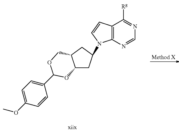
Scheme 9: Alternate route to of 4,5-disubstituted ((1S,2S,4R)-2-hydroxy-4-(7H-pyrrolo[2,3-d]pyrimidin-7-yl)cyclopentyl)methyl sulfamates
