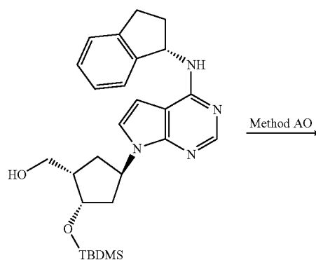
Scheme 15: Synthesis of ((1S,2S,4R)-2-{[tert-butyl(dimethyl)silyloxy]-4-{4-[(1S)-2,3-dihydro-1H-inden-1-ylamino]-7H-pyrrolo[2,3-d]pyrimidin-7-yl}cyclopentyl)methyl methanesulfonate
