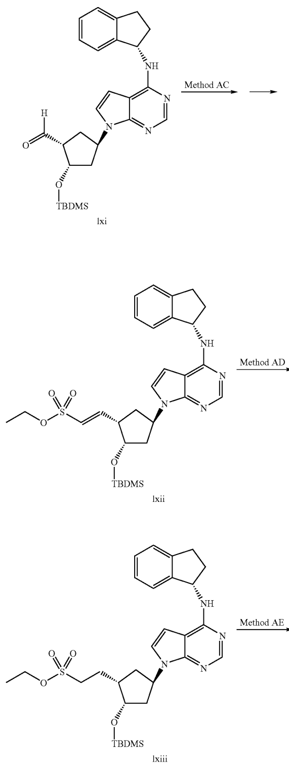
Scheme 11: Synthesis of 2-(((1S,2S,4R)-4-4-[(1S)-2,3-dihydro-1H-inden-1-ylamino]-7H-pyrrolo[2,3-d]pyrimidin-7-yl-2-hydroxycyclopentyl)ethanesulfonamide
