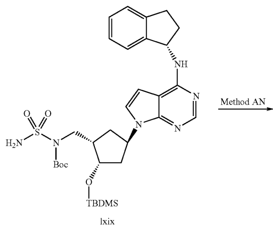
Scheme 14: General route to 4-substituted ((1S,2S,4R)-2-hydroxy-4-{7H-pyrrolo[2,3-d]pyrimidin-7-yl}cyclopentyl)methylsulfamides
