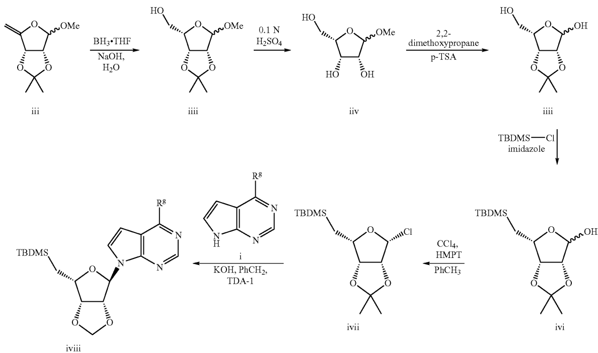
Scheme 10: Synthesis of ((2S,3S,4R,5R)-5-(4-(alkylamino)-7H-pyrrolo[2,3]pyrimidin-7-yl)-3,4-dihydroxy-tetrahydrofuran-2-yl)methyl sulfamates
