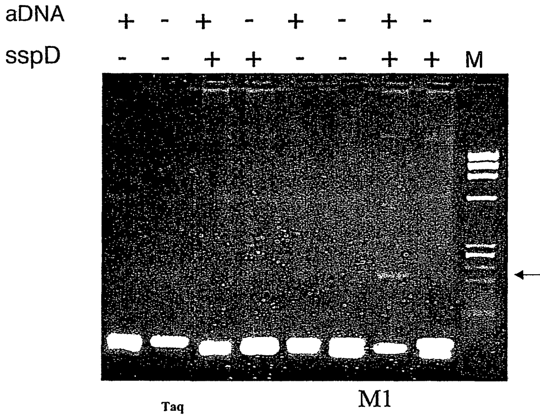
PCR amplification of a mix of extracts of cave hyenas ( Crocota spelea ) that had not previously produced an amplification product.
