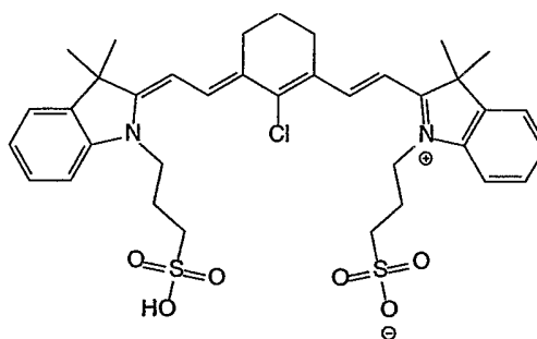
Dye structure:
