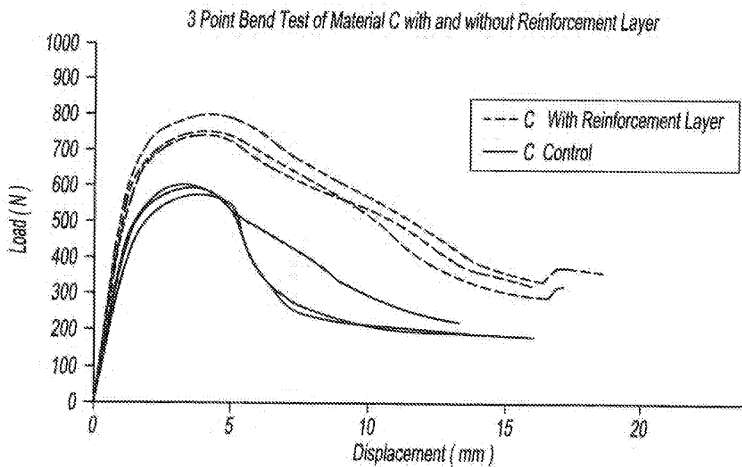
Flexural Testing Load Displacement Curves for Material C
