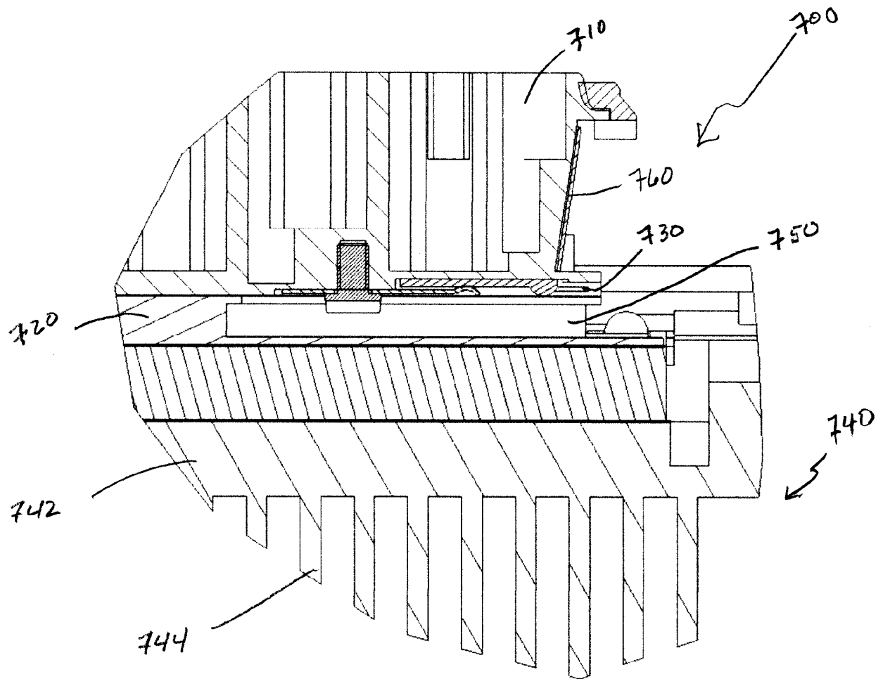
DETAIL A
