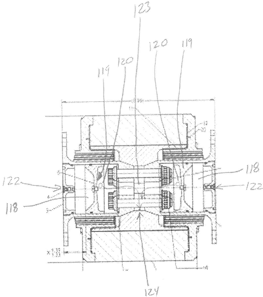
Section C-C
