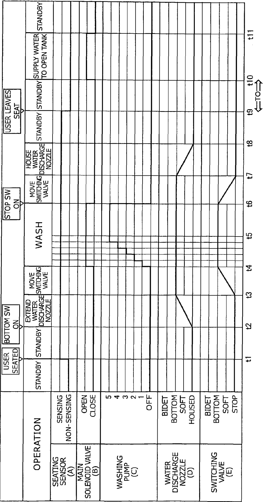
WASHING OPERATION TIMING CHART
