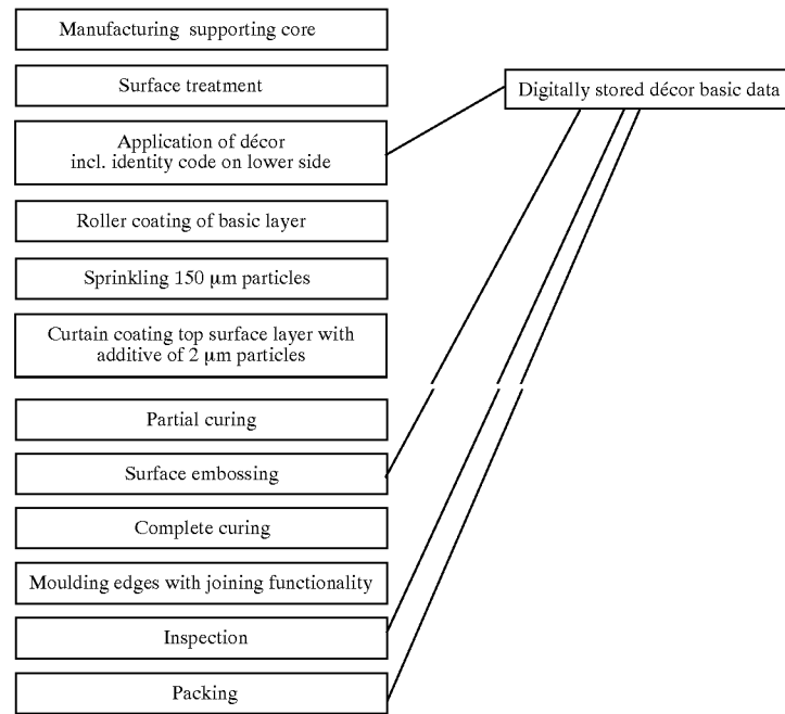
Process scheme 2.
