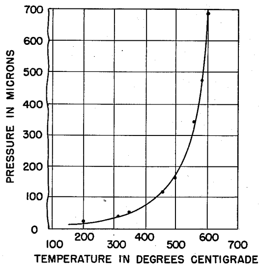
EXPERIMENTAL HYDROGEN PRESSURE-TEMPERATURE CURVE FOR ZIRCONIUM HYDRIDE
