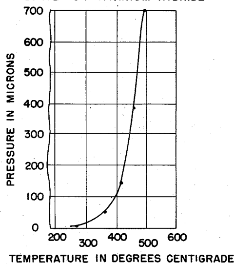
EXPERIMENTAL HYDROGEN PRESSURE-TEMPERATURE CURVE FOR TITANIUM HYDRIDE
