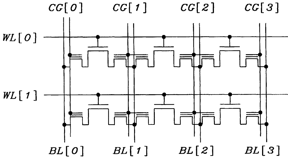
FIG. 4C - Prior Art
