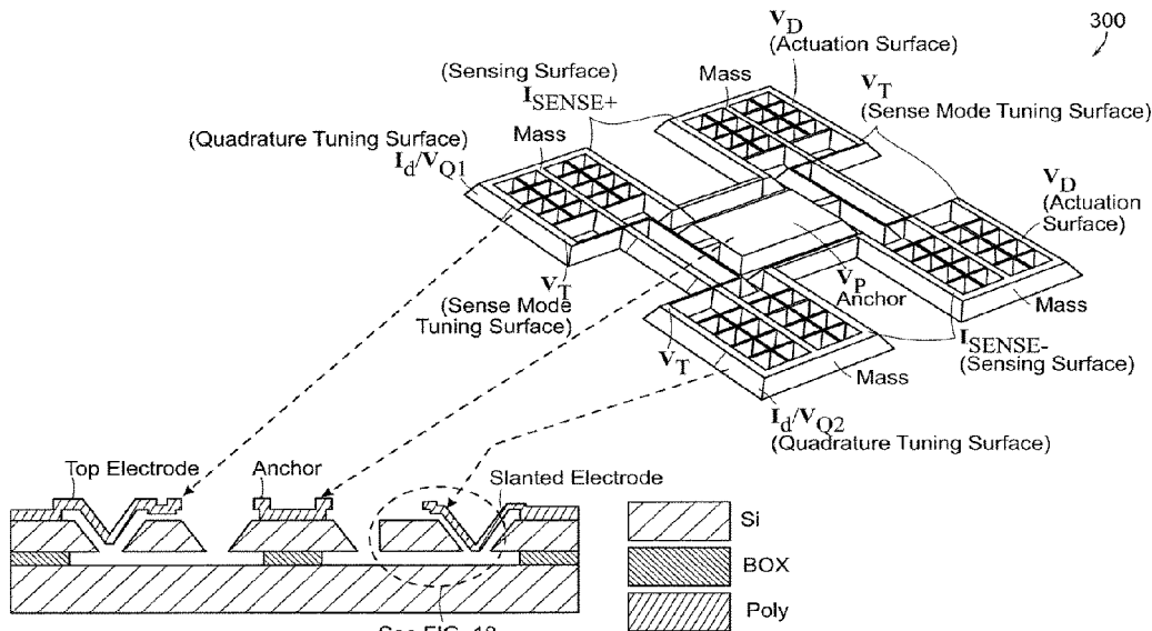
Cross-section-view including electrodes
