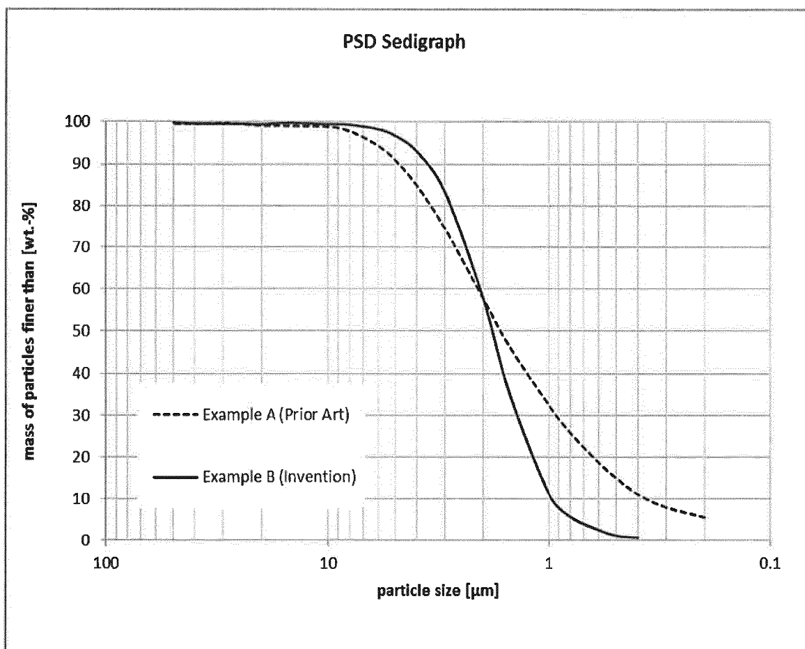
Fig. 1: PSD Sedigraph, examples A-B.
