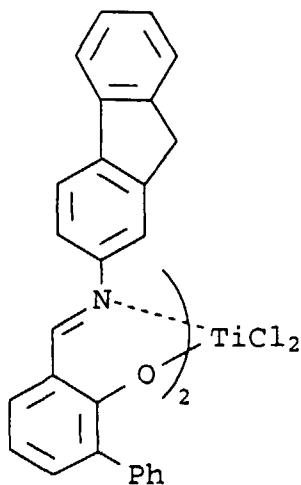
Compound A-17
