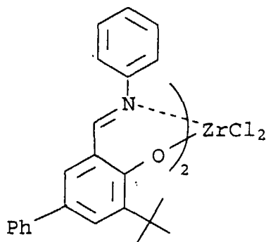
Compound B-14
