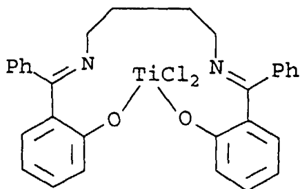
Compound A-36
