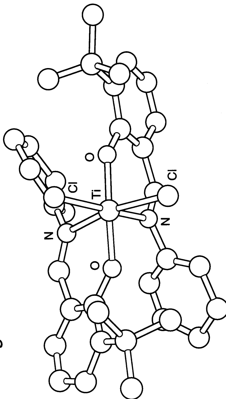
Structure of Compound A-1 from X-ray crystal structure analysis
