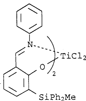
Compound A-15
