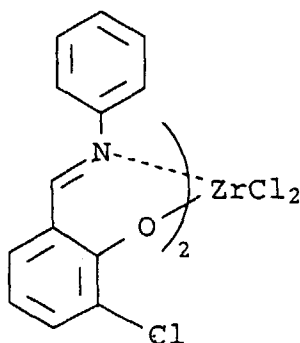
Compound B-31
