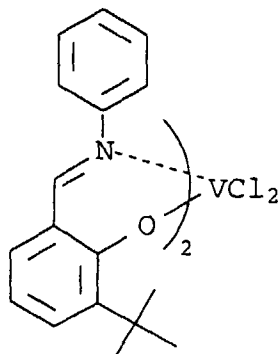
Compound D-1
