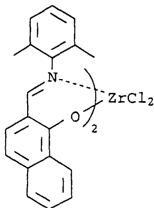
Compound B-5
