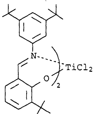
Compound A-28
