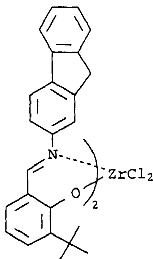
Compound B-8
