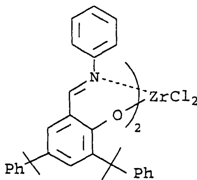
Compound B-12
