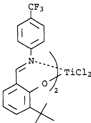
Compound A-21
