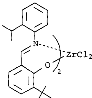
Compound B-27
