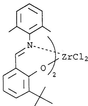
Compound B-20
