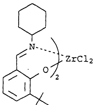
Compound B-25
