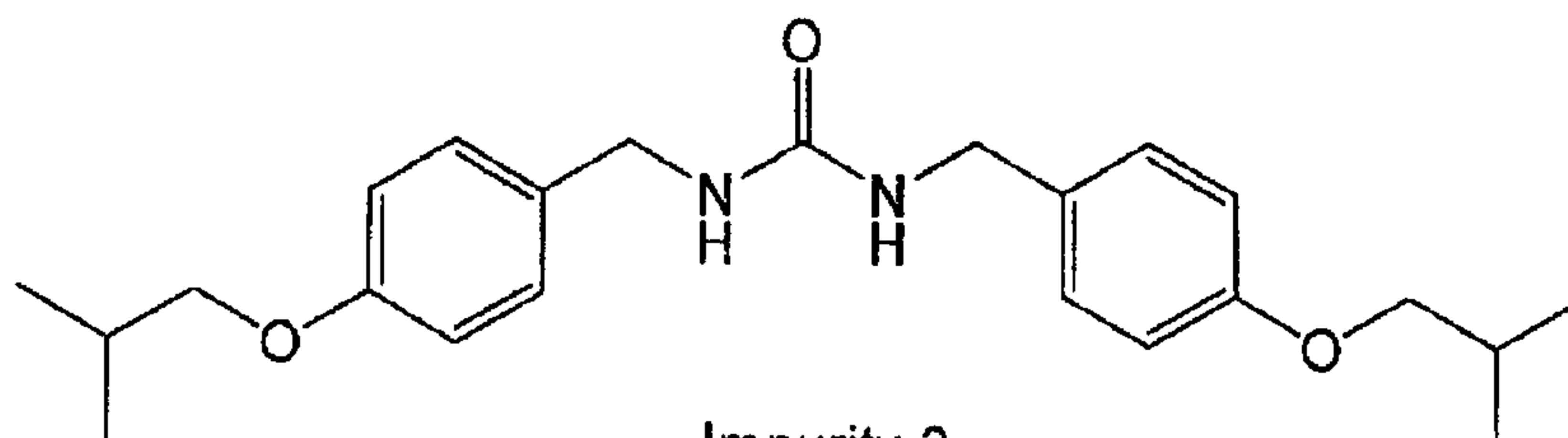
Impurity 2
