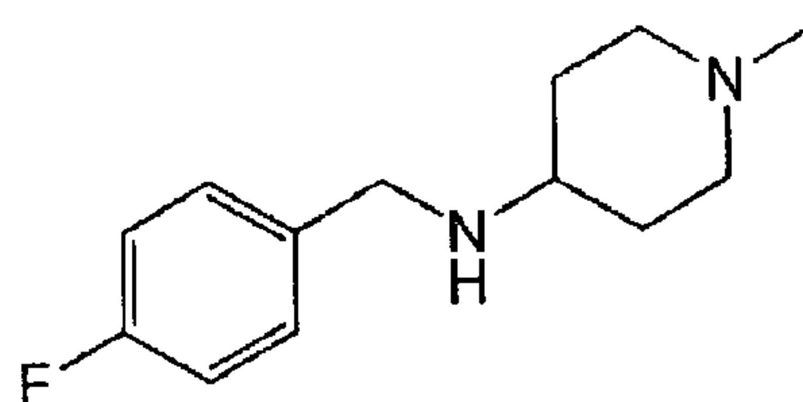
Impurity 1
