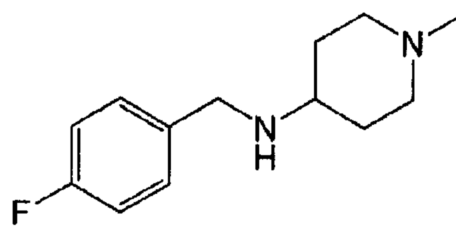
Impurity 1
