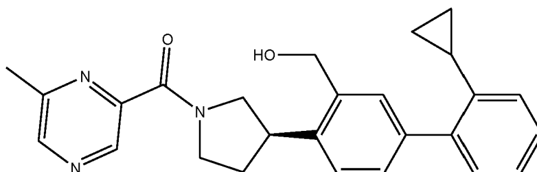
[3-(2'-Cyclopropyl-3-hydroxymethyl-biphenyl-4-yl)-pyrrolidin-1-yl]-(6-methyl-pyrazin-2-yl)-methanone (denoted herein: KM-032-E1 or compound E)
