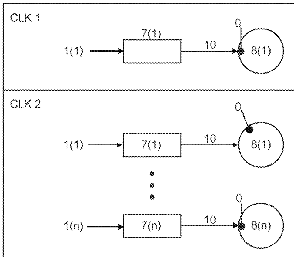
Figure 4: Skewed FIFO Buffers (Prior Art)
