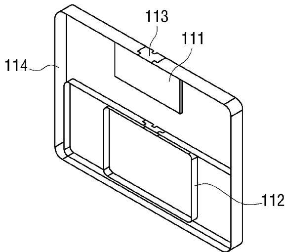
<CONFIGURATION OF RESONATOR>
