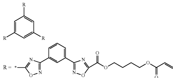
Disk-like liquid crystal compound D2
