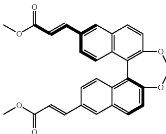
Polymerizable compound P1
