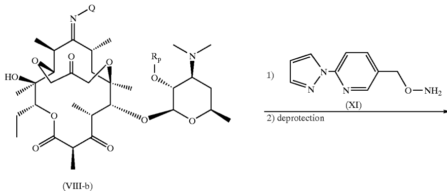
Scheme 4
