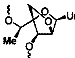
S-5'-Me-alpha-L-LNA
