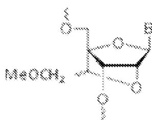
(R,S)-cMOE
