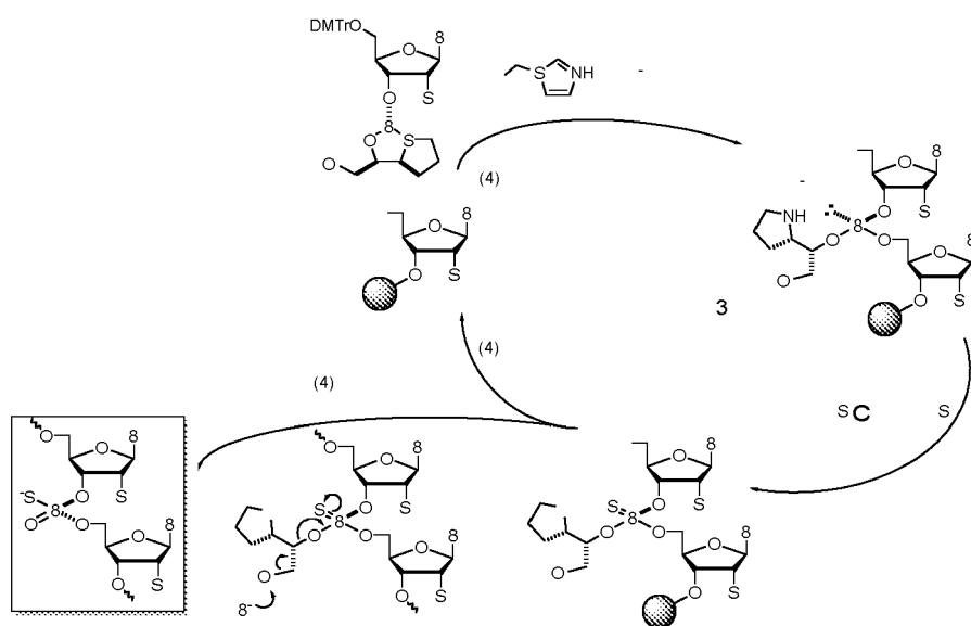
Scheme I-e. Example cycle using DPSE chiral auxiliary.
