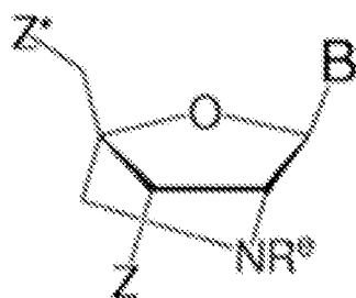
D-thio-LNA
