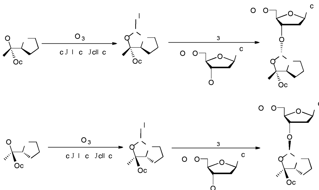
Scheme II. Example synthesis of coupling partner.
