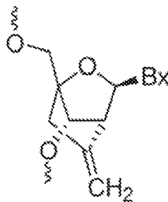
Methylene-cLNA
