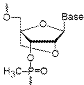
methylphosphonate-LNA
