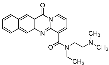
compound 2 (LI-326);
