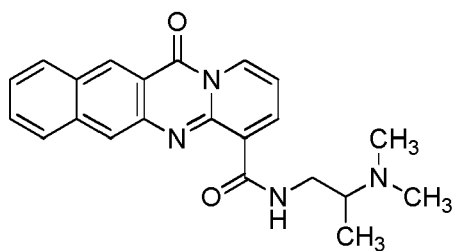
compound 28 (LI-409);
