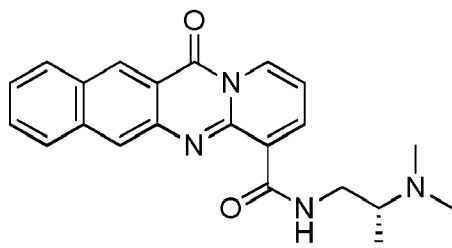
compound 34 (LI-621);
