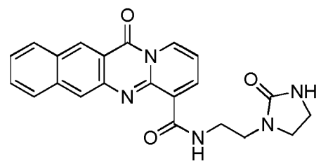
compound 6 (LI-277);
