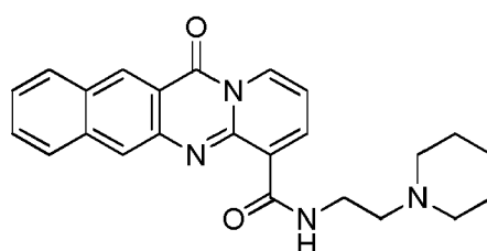
compound 23 (LI-218);
