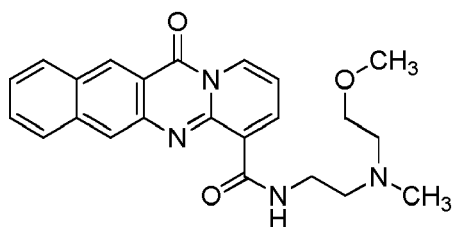
compound 26 (LI-412);
