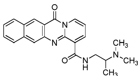
compound 28;
