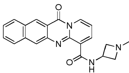
compound 29 (LI-613);
