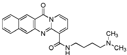
compound 10;
