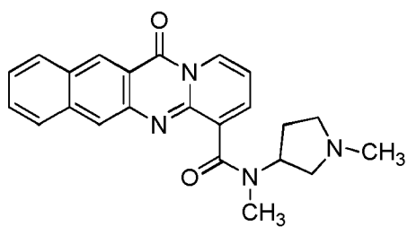
compound 17 (LI-340);
