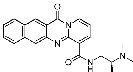
compound 36;
