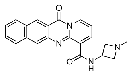
compound 29;
