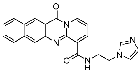
compound 3;
