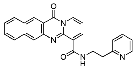
compound 4 (LI-248);
