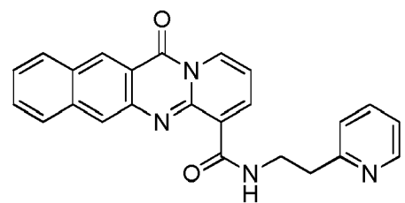
compound 4 (LI-248);
