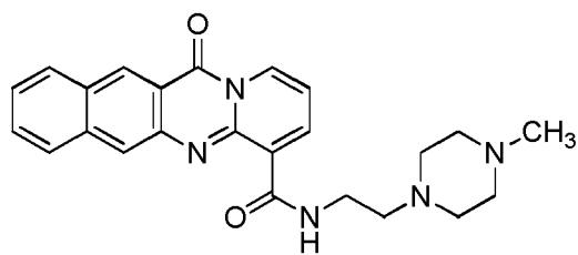
compound 25;
