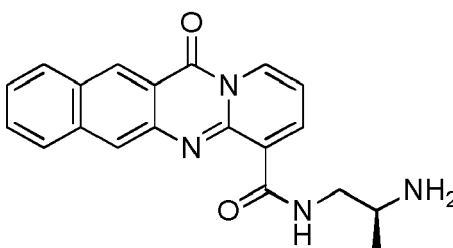
compound 35 (LI-622);
