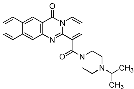
compound 16 (LI-360);
