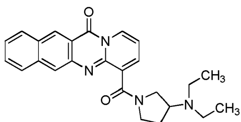
compound 19 (LI-329);
