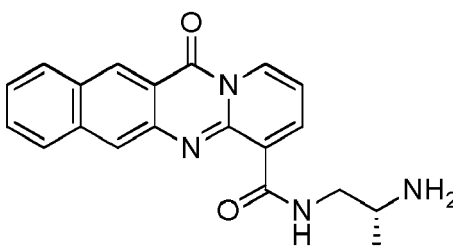
compound 33 (LI-620);
