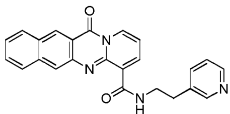
compound 5 (LI-247);
