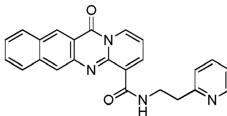
compound 4;
