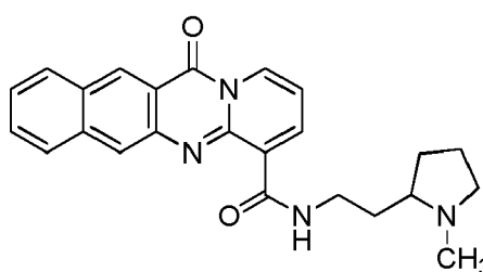
compound 11 (LI-281);
