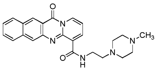
compound 25 (LI-258);
