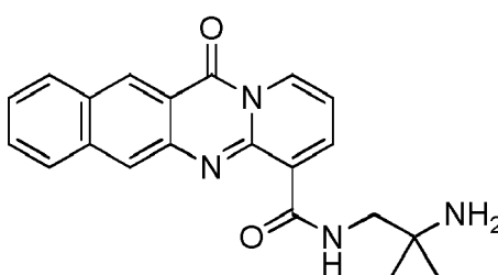
compound 30;
