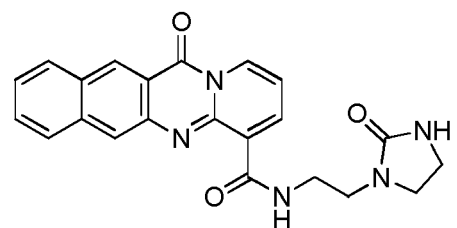
compound 6 (LI-277);
