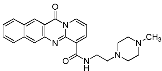
compound 25 (LI-258);
