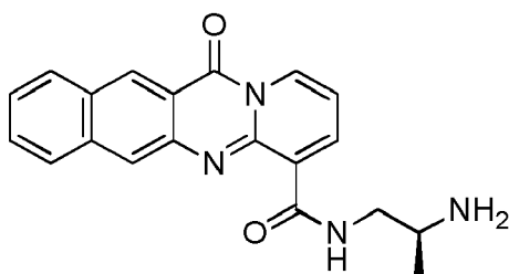
compound 35 (LI-622);
