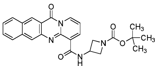
compound 15 (LI-363);
