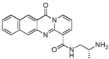
compound 33 (LI-620)
