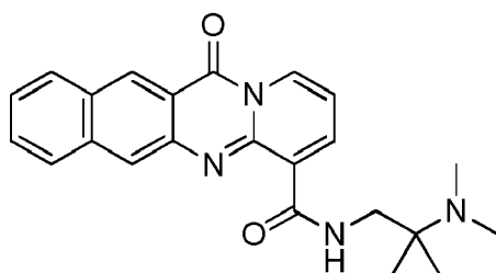
compound 31 (LI-615);
