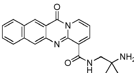
compound 30;
