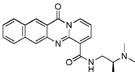
compound 36; and
