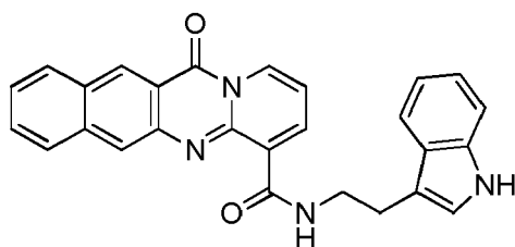
compound 7;
