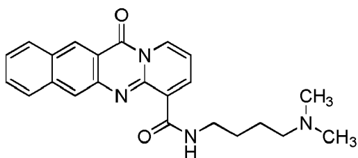
compound 10 (LI-280);
