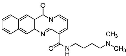
compound 10 (LI-280);
