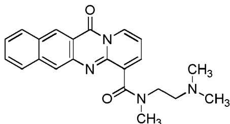
compound 1;
