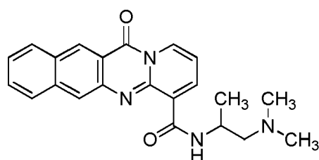
compound 27;
