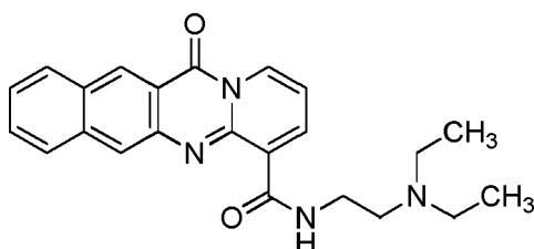
compound 20 (LI-325);
