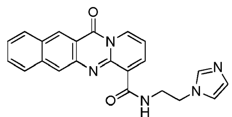
compound 3 (LI-279);
