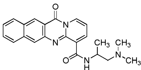
compound 27 (LI-344);
