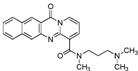
compound 12 (LI-343);
