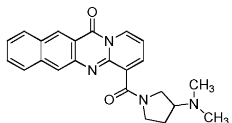
compound 18 (LI-330);
