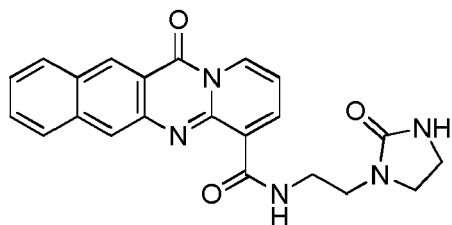
compound 6;
