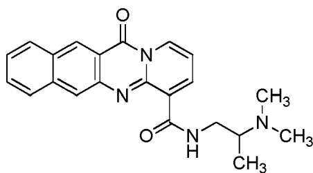
compound 28 (LI-409);
