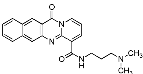
compound 9 (LI-220);
