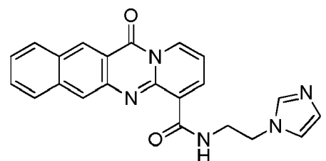
compound 3 (LI-279);
