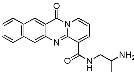
compound 32 (LI-619);
