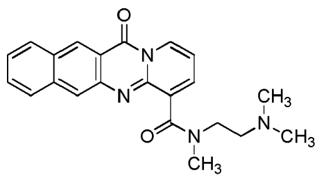
compound 1 (LI-361);
