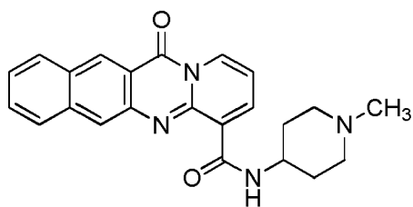
compound 13 (LI-257);
