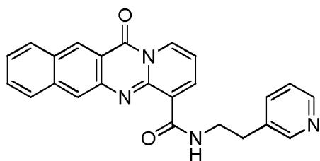
compound 5;
