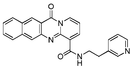
compound 5 (LI-247);
