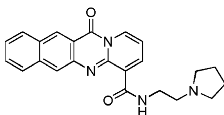
compound 22 (LI-278);
