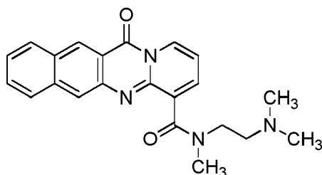
compound 1;
