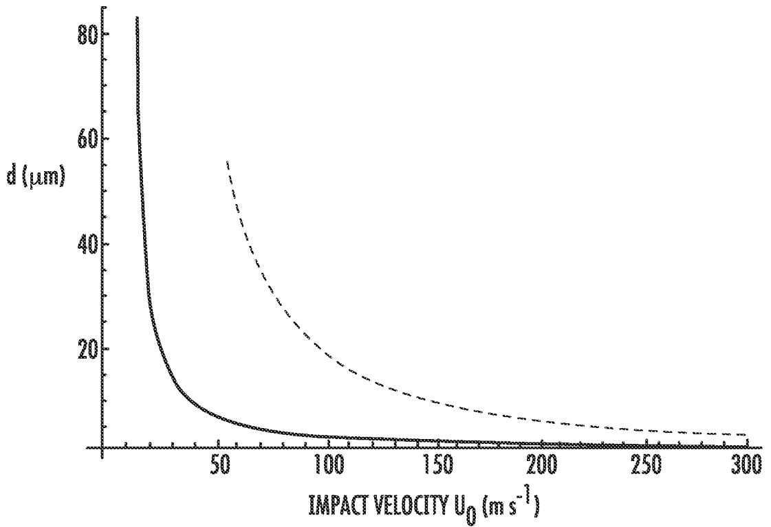
CRITICAL DIAMETER FOR SPLASHING TO OCCUR ON BAFFLE
