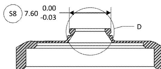
Section B-B Scale 3:1
