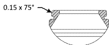
Detail D Scale 4:1
